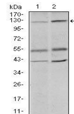
Western blot analysis of PC-3 (Lane 1) P...
