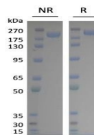
SARS-CoV-2 BA.2.75 Spike Trimer Protein
