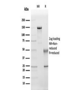
SDS-PAGE analysis of purified, BSA-free ...
