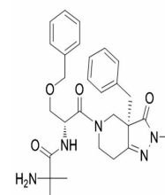
Chemical structure of Capromorelin
