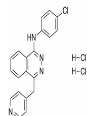
Chemical structure of Vatalanib
