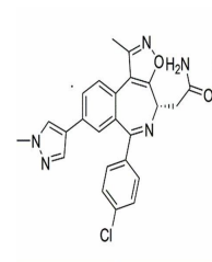
Chemical structure of BET bromodomain in...
