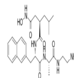
Chemical Structure of TAPI-1
