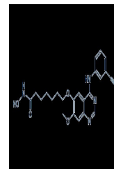
Chemical structure of CUDC-101
