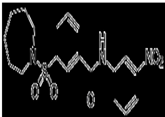
Chemical structure of SIRT2 Inhibitor II, AK-1
