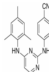
Chemical structure of Dapivirine
