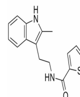
Chemical structure of CK-636
