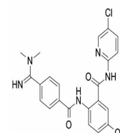
Chemical structure of Betrixaban
