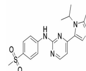
Chemical structure of AZD5438
