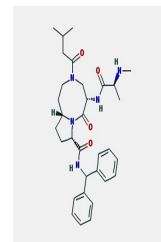
Chemical structure of AT-406
