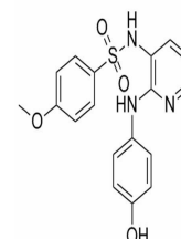
Chemical structure of ABT-751(E 7010)
