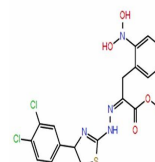
Chemical structure of 4EGI-1
