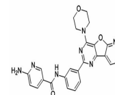
Chemical structure of YM201636
