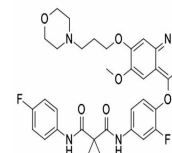
Chemical structure of Foretinib (GSK1363...
