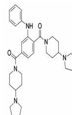
Chemical structure of UNC-1215
