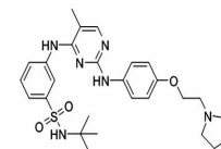
Chemical structure of TG101348(Fedratini...
