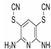
Chemical structure of PR-619
