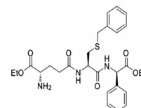
Chemical structure of Ezatiostat(TER199;...
