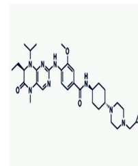
Chemical structure of Volasertib(BI6727)
