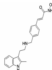
Chemical structure of Panobinostat(LBH58...
