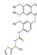
Chemical structure of Ki20227
