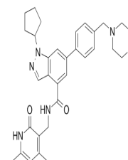
Chemical structure of EPZ005687.
