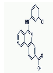
Chemical structure of CX-4945 (Silmitase...)
