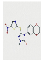
Chemical structure of BI-78D3
