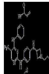
Chemical structure of CNX-2006
