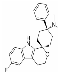
Chemical structure of Cebranopadol(GRT- 6...
