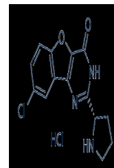
Chemical structure of BMS-863233 (XL-413...)
