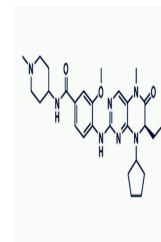
Chemical structure of Bi 2536
