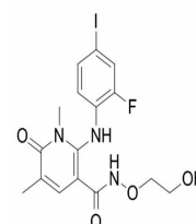
Chemical structure of AZD8330(ARRY-42470...
