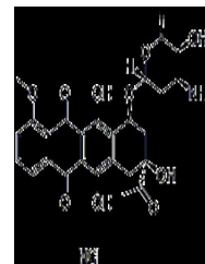
Chemical structure of Daunorubicin HCL
