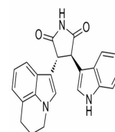
Chemical structure of Tivantinib (ARQ 19...)
