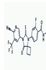
Chemical structure of ARN509
