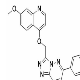
Chemical structure of AMG-208
