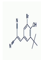
Chemical structure of AG-1024 (Tyrphosti...
