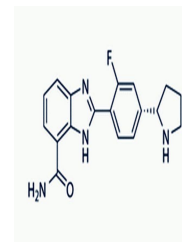
Chemical structure of A-966492
