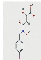
Chemical structure of BMS-538203
