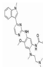
Chemical structure of Mereletinib (AZD-9...)
