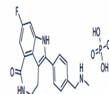
Chemical structure of Rucaparib phosphat...
