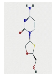
Chemical structure of Apricitabine
