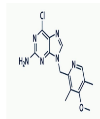
Chemical structure of BIIB021(CNF2024)
