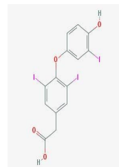
Chemical structure of Tiratricol
