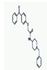
Chemical structure of AdipoRon
