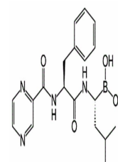
Chemical structure of Bortezomib (Velcade...)
