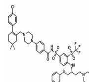
Chemical structure of ABT-263 (Navitoclax...)
