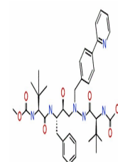
Chemical structure of Atazanavir
