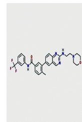
Chemical structure of AMG-47a
